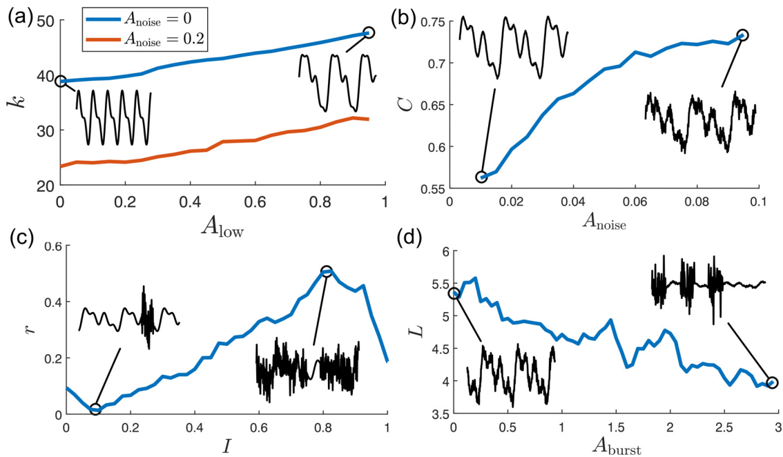
FIG. 3. Visibility parameters of the synthetic time-series: (a) average degree K with respect to the amplitude of the lowest frequency component of the time-series A_{low} ; (b) clustering coefficient C with respect to the amplitude of noise A_{noise} ; (c) assortativity r with respect to the intermittency I ; and (d) average path length L with respect to the amplitude A_{burst} of localized bursts ( I = 0.33 ). Relevant time-series are plotted as insets.
