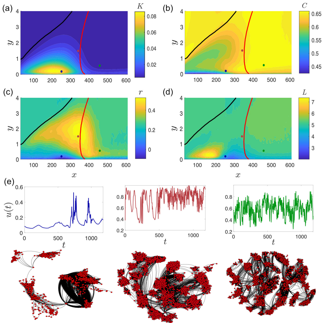
FIG. 4. Visibility graph measures in the transitional boundary layer: (a) Average degree, (b) clustering coefficient, (c) assortativity, and (d) average path length. The boundary layer height \delta_{99} is shown in black, while the average position of the TNTI \bar{x}_{\text{TNTI}}(y) is shown in red. Panel (e) shows three time-series sampled at the corresponding, color-coded points of the domain; the spanwise coordinate is z = 13.95 for all time-series. Below each time-series, the corresponding visibility graph is drawn by a force-directed algorithm.
